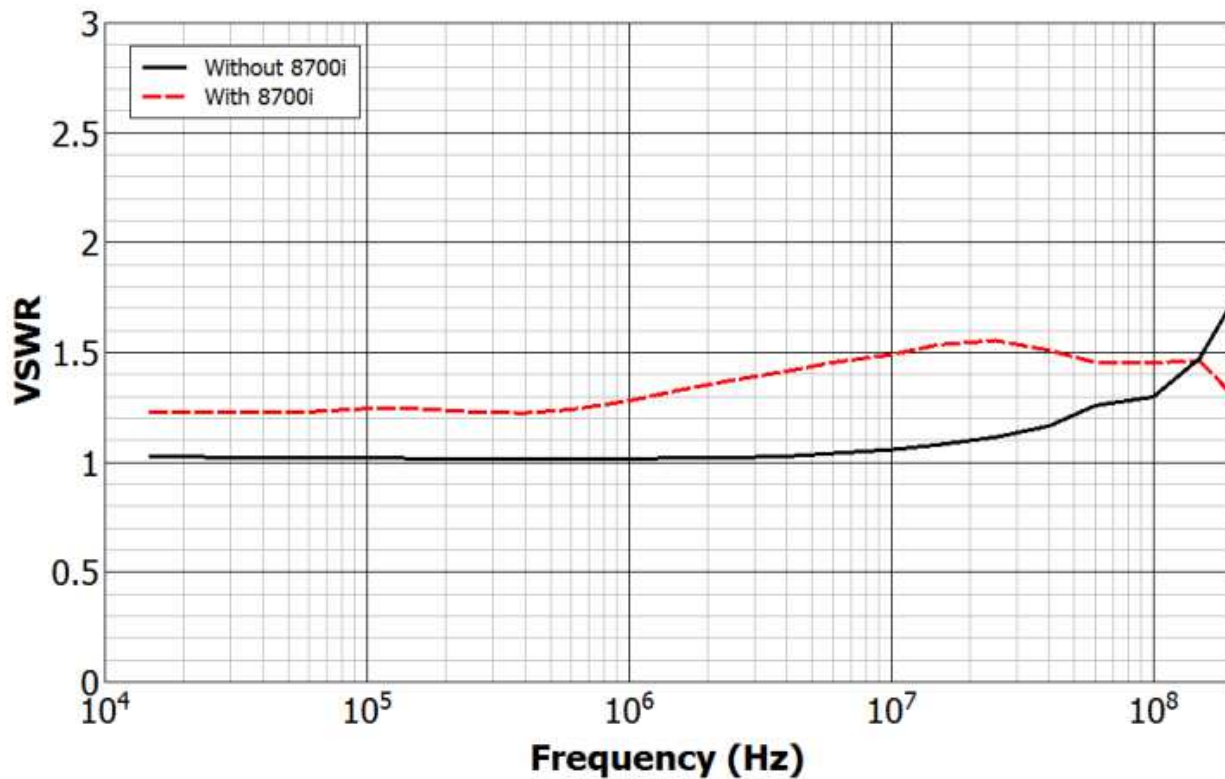
F-3 Calibration Fixture VSWR
